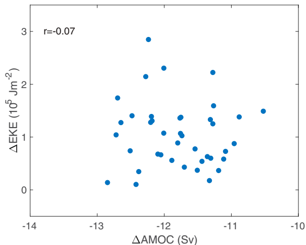
FIG. 9. The response to anthropogenic emissions of DJF North Atlantic TEKE ( 10^5 \text{ J m}^{-2} ) averaged over the downstream region of the storm track as a function of the AMOC response (Sv; 1 \text{ Sv} \equiv 10^6 \text{ m}^3 \text{ s}^{-1} ) in LE. Their correlation appears in the upper-left corner.
