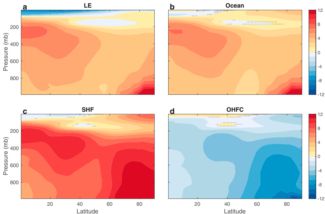
FIG. 7. As in Fig. 4, but for the mean temperature averaged over the downstream region of the storm track ( 60^{\circ}\text{W} – 30^{\circ}\text{E} ).
